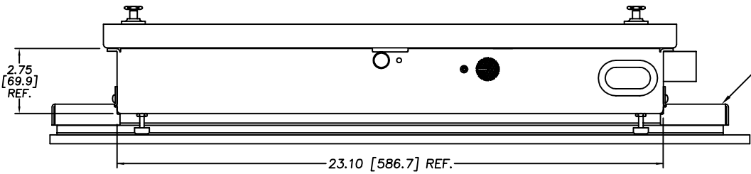
DETAIL A
