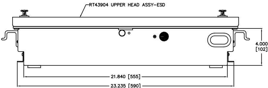
RT43904 UPPER HEAD ASSY-ESD
